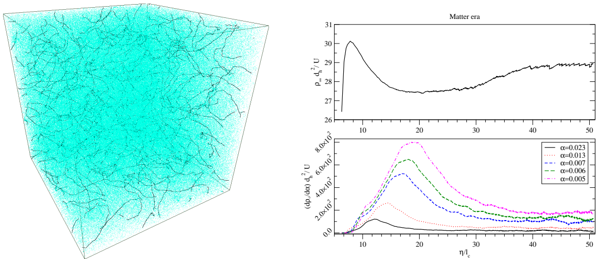
Figure 1: Left panel: A typical string loop distribution according to the latest simulation by Ringeval et al. (2007) during the matter era. The observable Universe occupies one eighth of the box, whose edge is 100\ell_c , with \ell_c being the correlation length of the Vachaspati-Vilenkin (1984) initial conditions. The right panel shows, for the same era, the evolution of the energy density associated with long strings (top) and loops (bottom) of physical sizes \ell_{\text{phys}} = \alpha d_h , d_h being the horizon size. The time variable is the rescaled conformal time \eta/\ell_c . These results show the network reaching scaling, as required.
