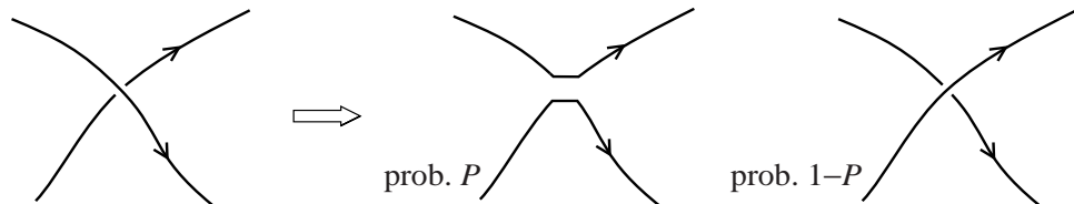
Figure 2: String intercommutation
