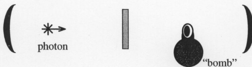
Fig.6 A purely interferometric interaction-free measurement system. In the absence of a bomb in the right cavity, a photon initially in the left cavity will with certainty be found in the right cavity after N cycles (where N depends on the precise value of the coupling beam splitter's reflectivity R ). With the bomb, and when N \geq 4 , the photon will more likely be found in the left cavity on the N th cycle. It is assumed that the cavity lengths are identical.
